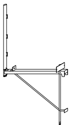
SUPPORTING BRACKET WITH GUARDRAIL
